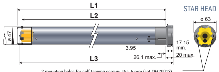
2 mounting holes for self tapping screws. Dia. 5 mm (cat #9670013). Depth 13 mm spaced 1.89" (48 mm) apart.
